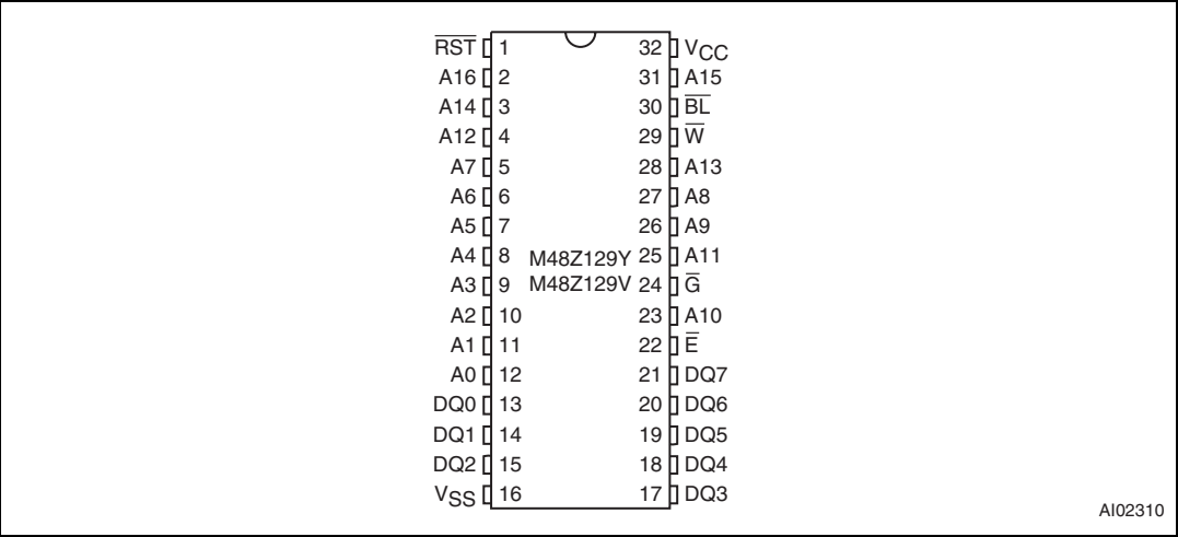
Figure 2. DIP connections
