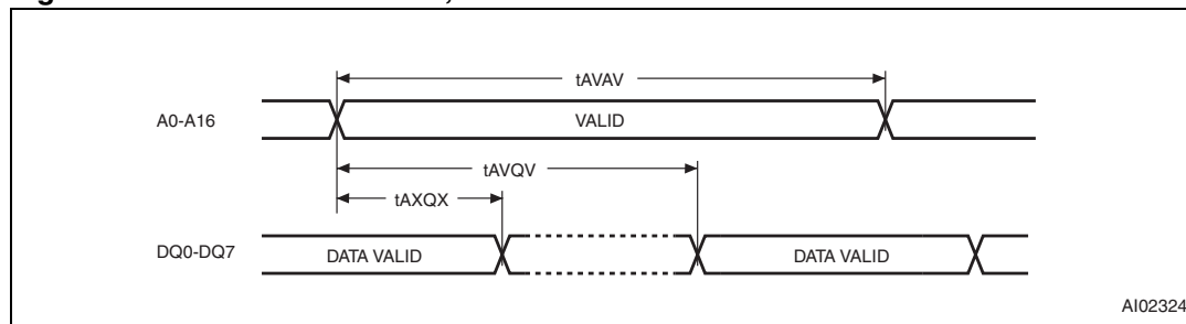
Figure 4. Address controlled, READ mode AC waveforms
